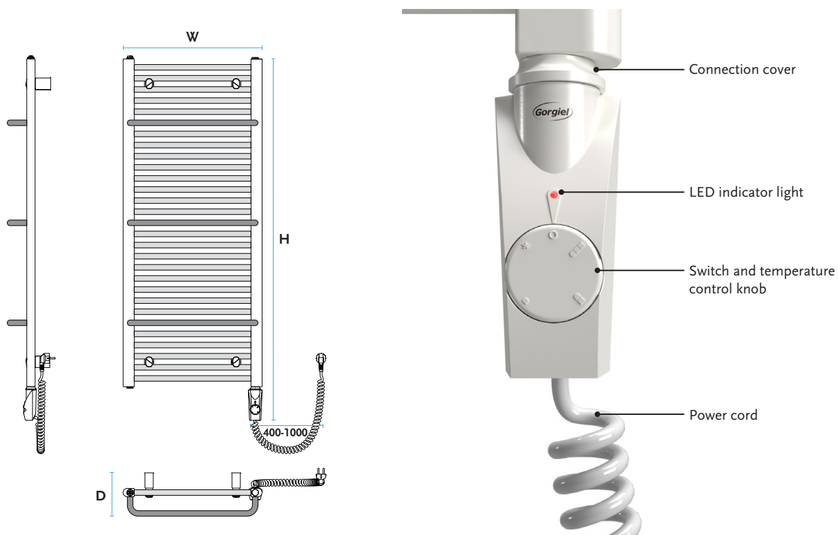
H - total height; Hg - radiator height; W - width; D - depth;
